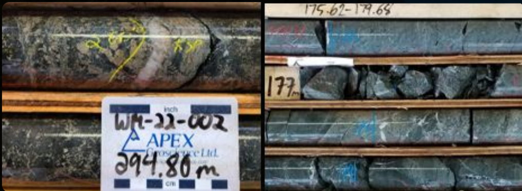
Left image: WM22-02 (left) clotty pyrite mineralized, chlorite-silica-potassium feldspar-magnetite altered volcanic (this sample 5.8 g/t Au and 787 ppm Cu); WM22-03 (right) brecciated and silica-flooded magnetite veined zone (this sample 9.9 g/t Au)
